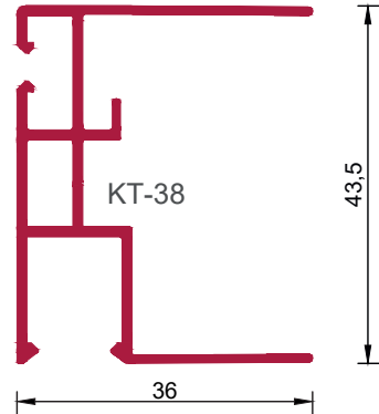
KT-38 3-000-340-X U = 298 mm VE = 4 Stangen
