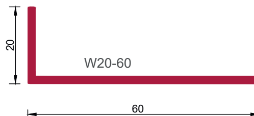
Montagewinkel W20-60 4-000-300-X VE = 8 Stangen
