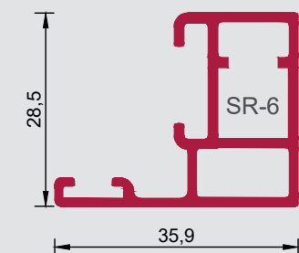
SR-6 5-000-180-X U = 185 mm VE = 4 Stangen
