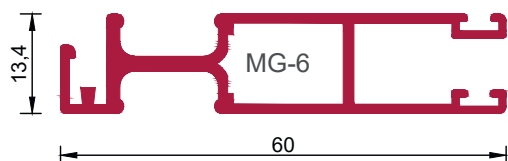
MG-6 6-000-105-X U = 251 mm VE = 8 Stangen
