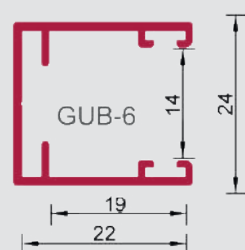
GUB-6 3-000-260-X U = 179 mm VE = 8 Stangen
