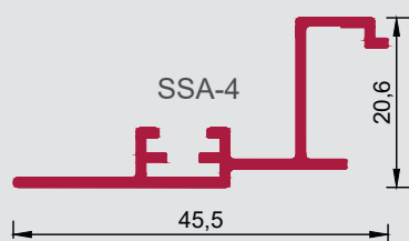
SSA-4 (Lagerlänge 450 cm) 5-000-255-X U = 201 mm VE = 6 Stangen
