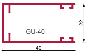
Standardführungs- schiene GU-40 3-000-240-X VE = 8 Stangen
