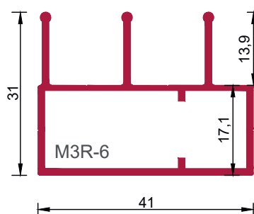
M3R-6 6-000-236-X U = 198 mm VE = 4 Stangen
