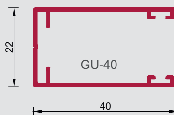
GU-40 (Lagerlänge 600 cm) 3-000-240-X U = 242 mm VE = 8 Stangen
