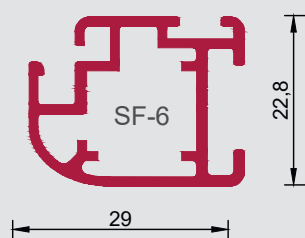
SF-6 5-000-100-X U = 155 mm VE = 4 Stangen
