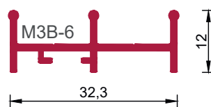
M3B-6 6-000-231-X U = 141 mm VE = 4 Stangen
