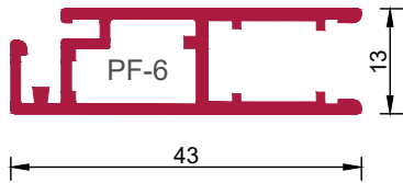
PF-6 2-000-500-X U = 189 mm VE = 8 Stangen
