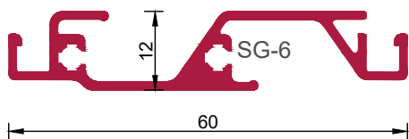
SG-6 2-000-140-X U = 250 mm VE = 6 Stangen
